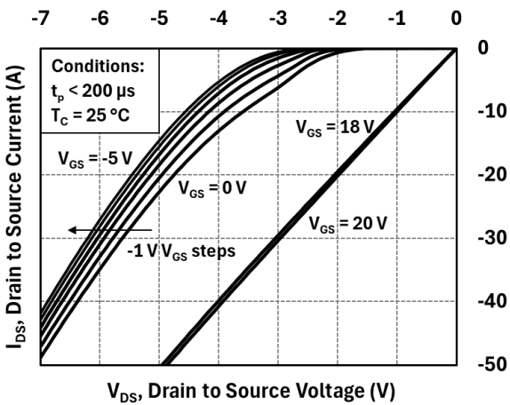
Figure 20: Body Diode Characteristics at 25 \text{ }^{\circ}\text{C}
