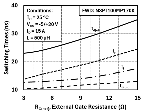
Figure 19: Switching Times vs. R_{G(ext)} ( V_{DD} = 1200 \text{ V} )
