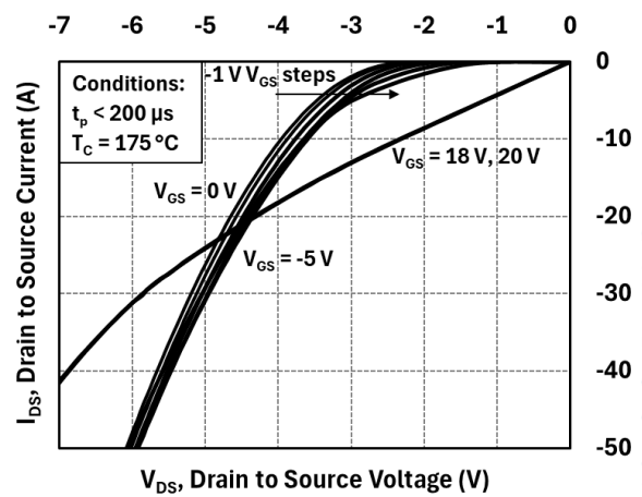
Figure 21: Body Diode Characteristics at 175 \text{ }^{\circ}\text{C}
