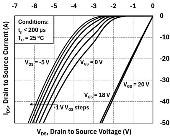
Figure 20: Body Diode Characteristics at 25\ ^{\circ}\text{C}
