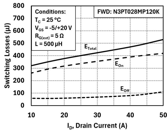
Figure 16: Inductive Switching Energy vs. Drain Current ( V_{DD} = 800 V)
