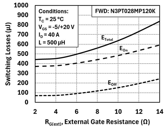
Figure 17: Inductive Switching Energy vs. R_{G(ext)} ( V_{DD} = 800 V)
