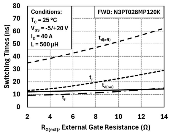
Figure 19: Switching Times vs. R G(ext) (V DD = 800 V)
