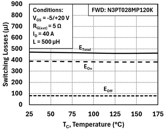
Figure 18: Inductive Switching Energy vs. Temperature (V DD = 800 V)
